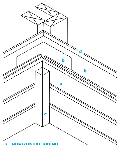
Figure 2: CORNER DETAILS
