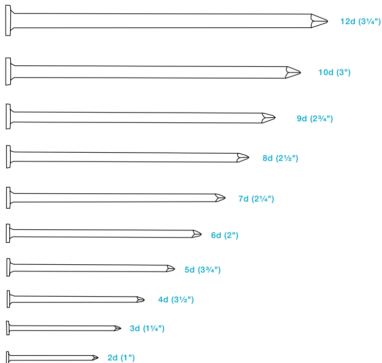
Figure 5: NAIL LENGTHS
